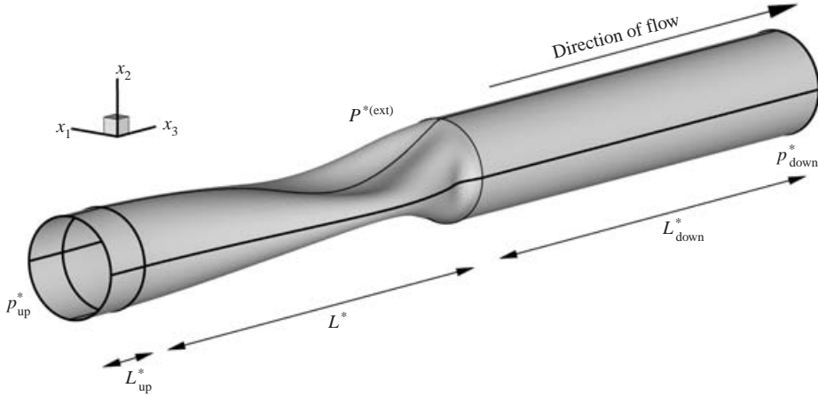
FIGURE 1. Sketch illustrating the coordinate system and the geometry of the collapsible tube. An elastic tube of lengths L^* is mounted on two rigid tubes of lengths L_{\text{up}}^* and L_{\text{down}}^* . The fluid pressure at the upstream end of the system ( x_3^* = -L_{\text{up}}^* ) is p_{\text{up}}^* ; the downstream fluid pressure (at x_3^* = L^* + L_{\text{down}}^* ) is p_{\text{down}}^* and the external pressure is P^{*(\text{ext})} . Note the small secondary buckling pattern at the downstream end of the elastic segment.
